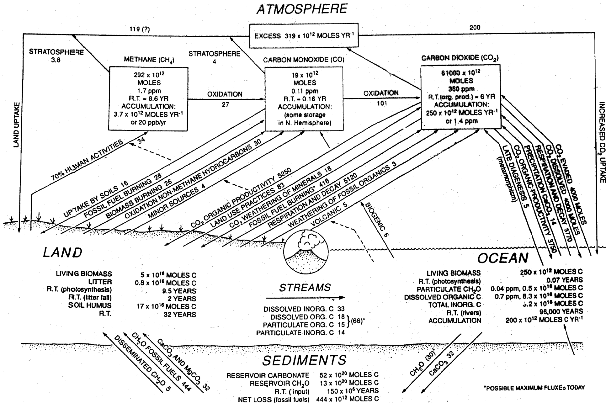
Figure 1. Global biogeochemical cycle of carbon. Fluxes in units of 10 12 moles C per year.
