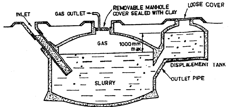
Figure 1 Fixed dome (Chinese) digester
