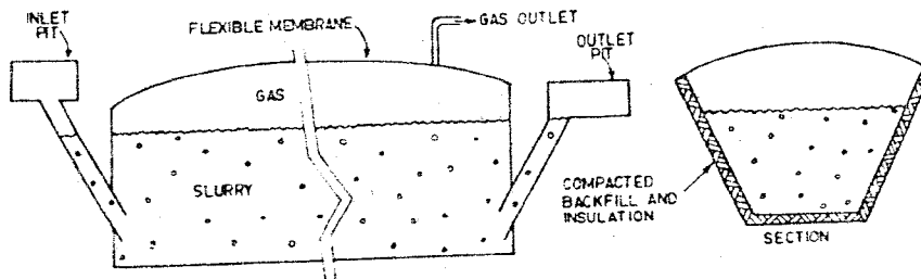
Figure 4 Plug flow digester
