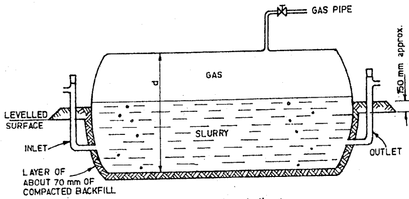
Figure 3 Bag (Taiwan) digester
