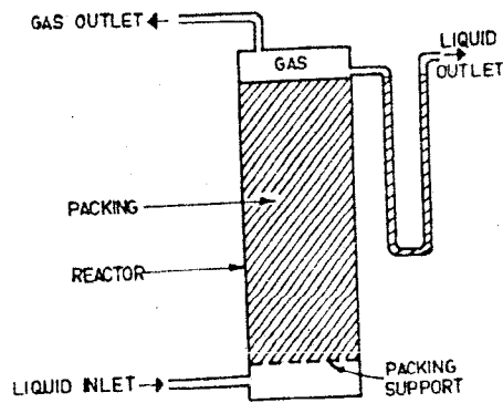
Figure 5 Anaerobic filter
